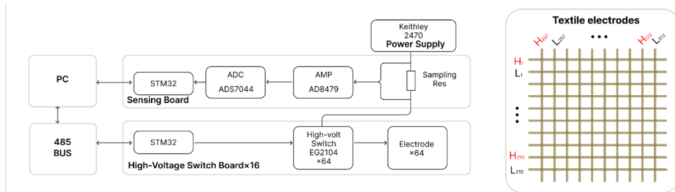
Figure 2: TacTex comprises the power supply, the sensing unit, the switches unit, and the textile electrodes.
