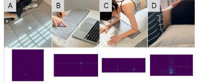
Figure 12: Example applications with visualizations of raw current data captured over the whole textile. A) Large-size TacTex interface with projected visual content. B) TacTex interface integrated into desk cloth. Example applications in embedded haptic display. C) TacTex interface embedded in a yoga pad. D) TacTex interface integrated into a pillow.
