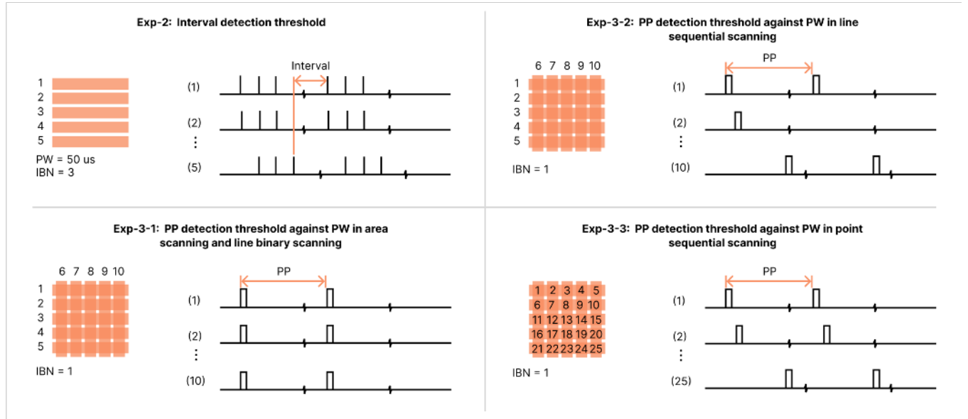
Figure 10: Electrical stimuli used in Exp-2 and Exp-3.
